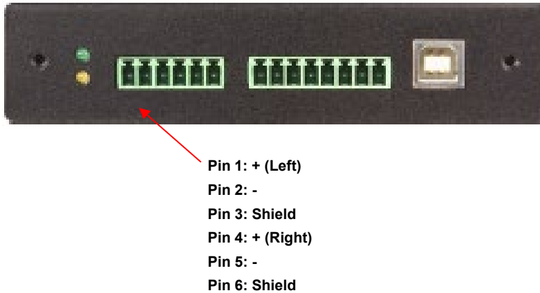
Figure 10. Audio Connector Pinout Diagram
