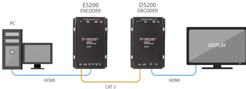
Figure 4. One Source to One Display Diagram
