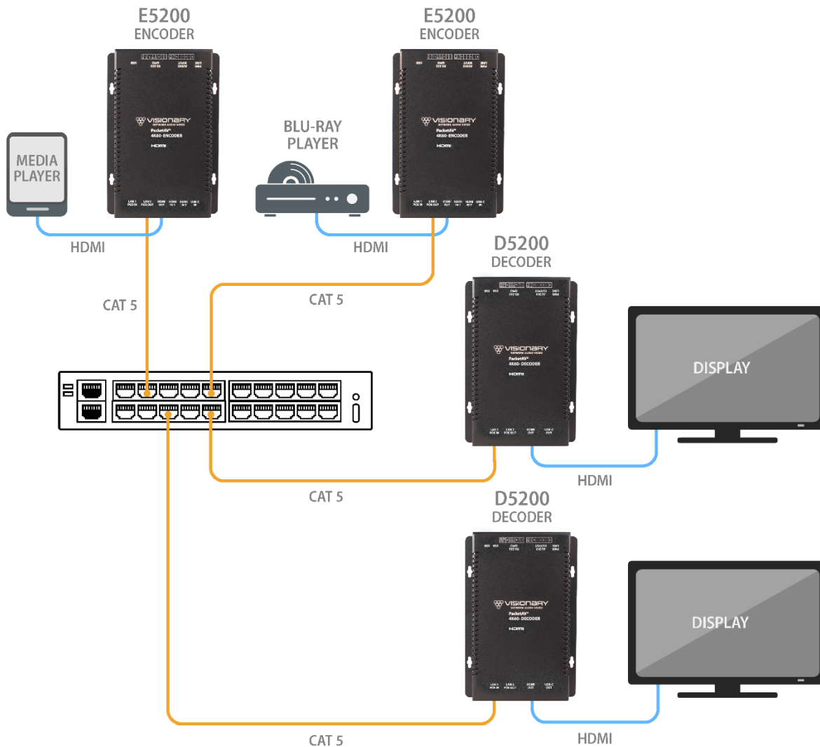
Figure 6. Many Sources to Many Displays Diagram
